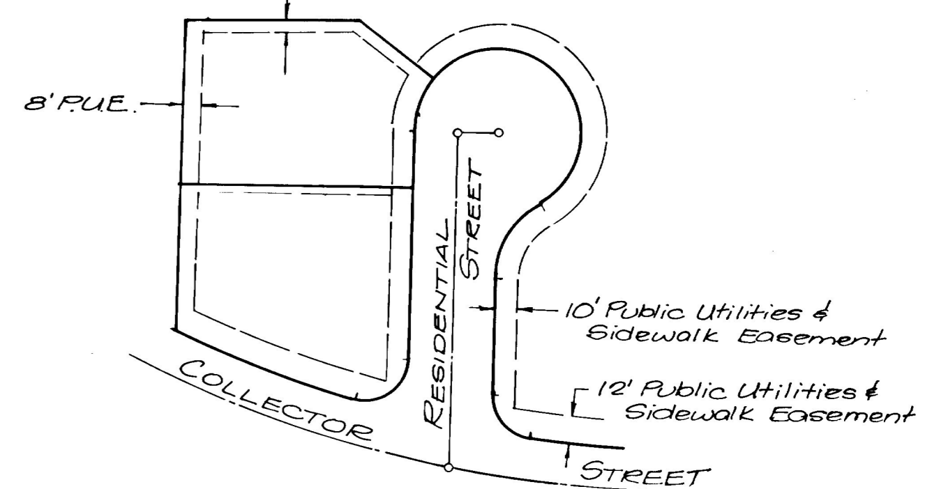
Public Utilities & Sidewalk Easement Detail (Typical)
