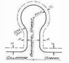
PUBLIC UTILITIES AND SEWERAGE EASEMENT DETAILS (Typical)
