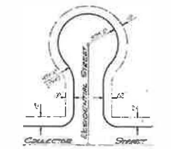
PUBLIC UTILITIES AND SIDEWALK EASEMENT DETAIL (TYPICAL)
